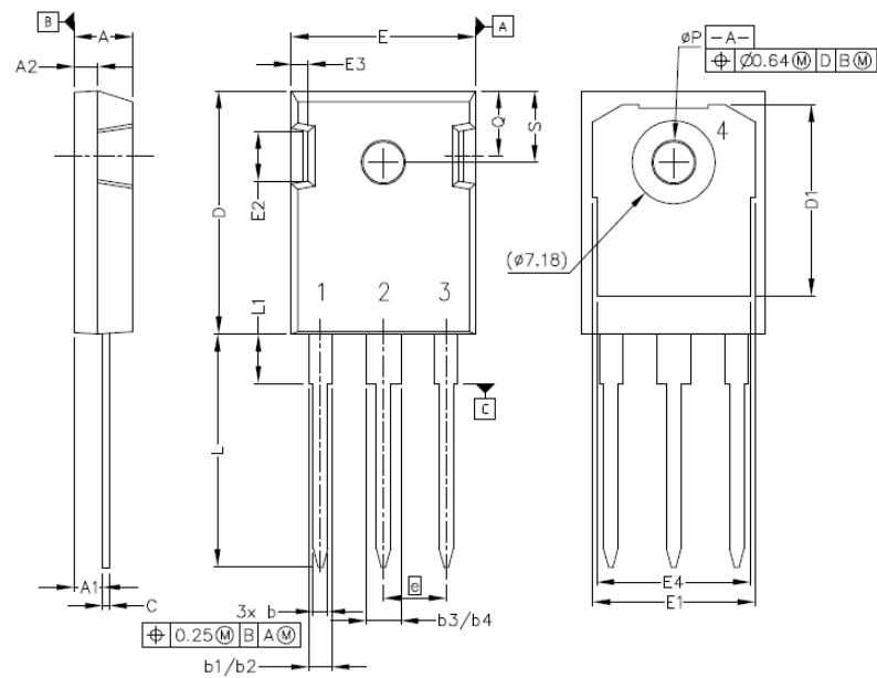
Package TO-247-3
