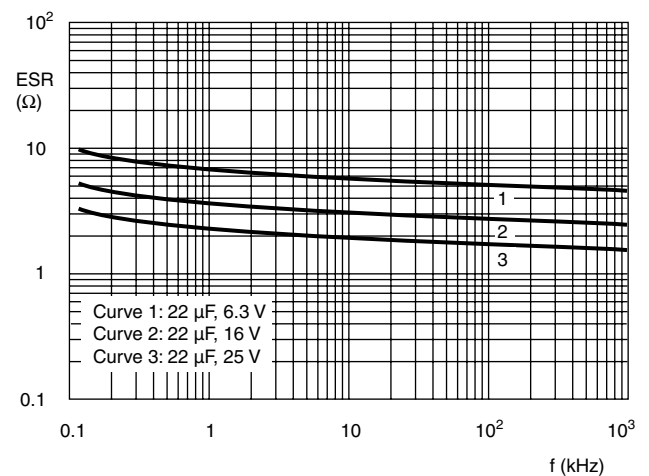
Fig.6 Typical ESR as a function of frequency at 20 ^{\circ}\text{C}
