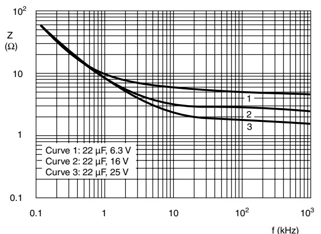
Fig.8 Typical impedance as a function of frequency at 20 ^{\circ}\text{C}
