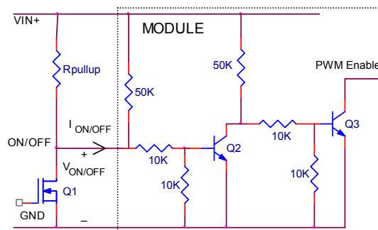
Figure 53. Circuit configuration for using positive On/Off logic.
