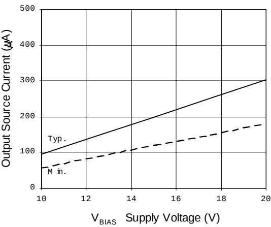
Figure 21B. Output Source Current vs. Supply Voltage
