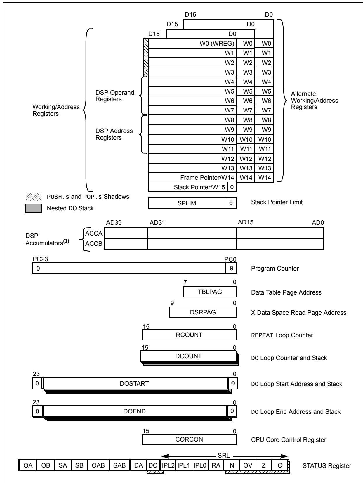
FIGURE 3-2: PROGRAMMER'S MODEL
