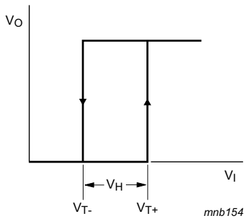
Fig 7. Transfer characteristic
