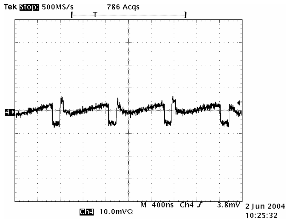
Figure 10. DC773 Constant Low-Ripple LED Current ( I_{LED} = 1000mA , V_{IN} = 3.6V , T_A = 25^\circ C ) CH4 is I_{LED} (AC) 20mA/10mVΩ
