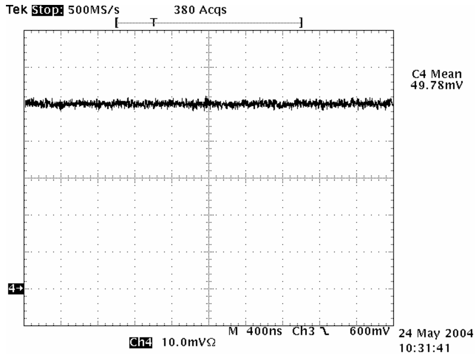
Figure 9. DC773 Constant Low-Ripple LED Current ( I_{LED} = 1000mA , V_{IN} = 3.6V , T_A = 25^\circ C ) CH4 is I_{LED} 200mA/10mVΩ
