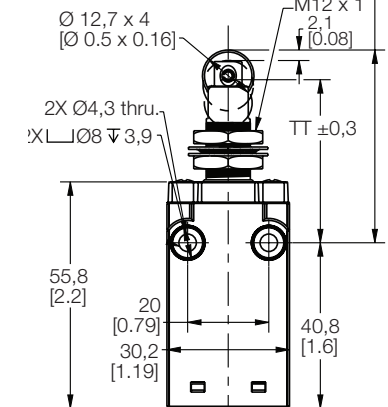
Figure 13. Panel-Mount Roller Plunger P Dimensions
