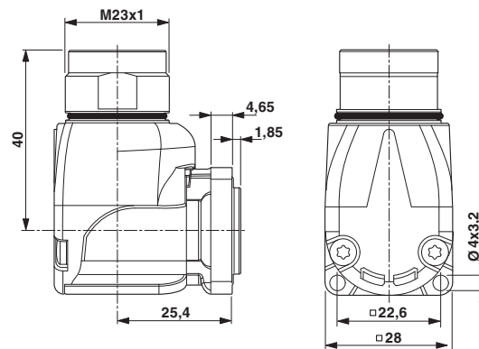
Dimensioned drawing
