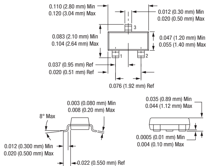
Figure 8. SOT-23 Package Dimension Drawing
