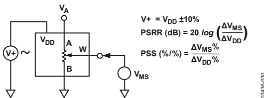
Figure 31. Test Circuit for Power Supply Sensitivity (PSS, PSSH)
