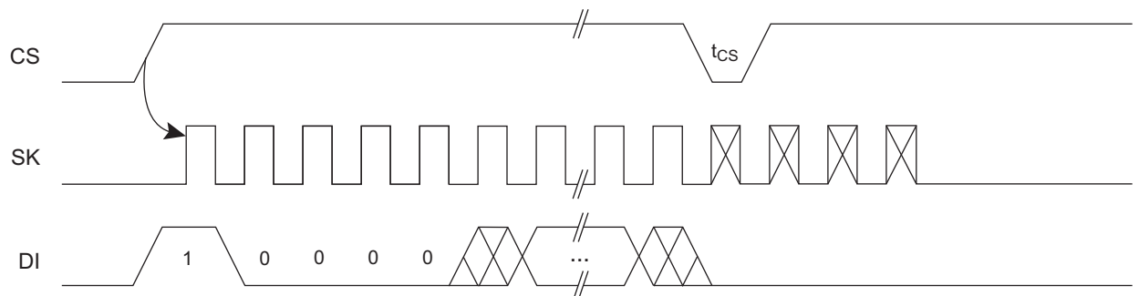
Figure 6-4. EWDS Timing
