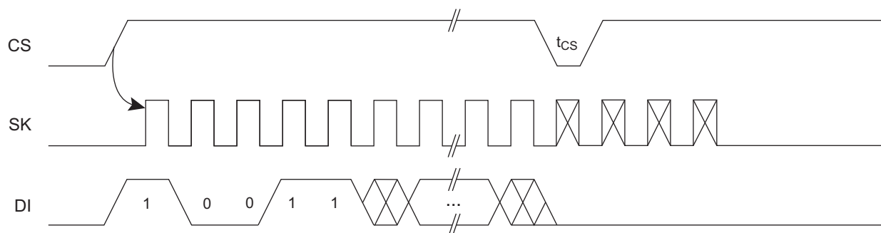
Figure 6-3. EWEN Timing
