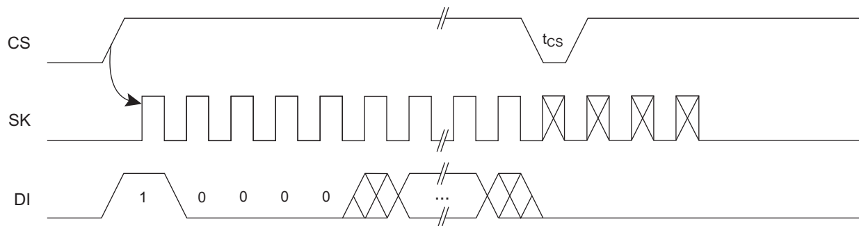
Figure 6-4. EWDS Timing
