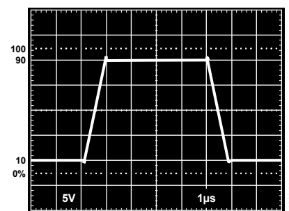
Figure 5. Excellent Output Drive, R_L = 600 \Omega
