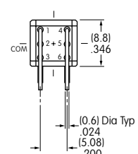
Double Pole
