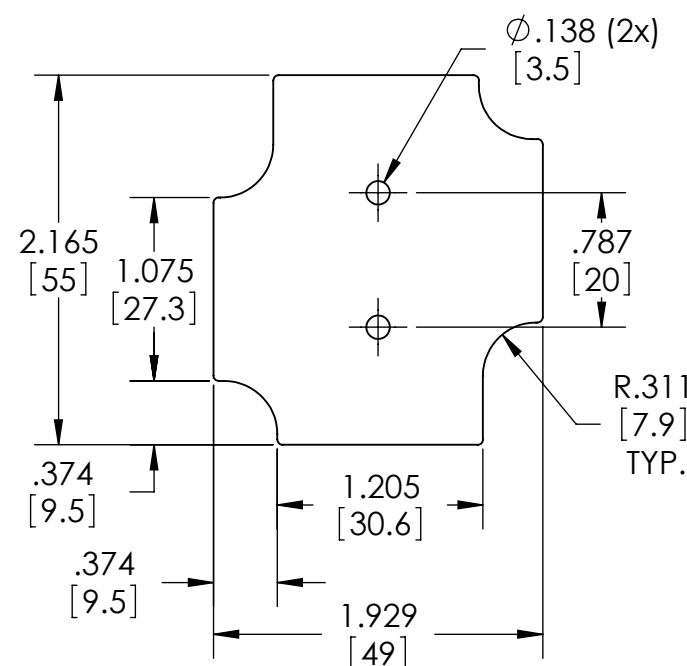
SUGGESTED PC BOARD LAYOUT
