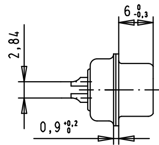
Solder bucket for AWG 20
