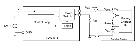
FIGURE 6-2: Constant Current Example.
