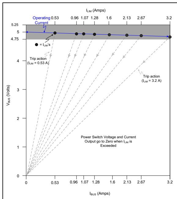
FIGURE 6-1: Current Limiting in Trip Mode.
