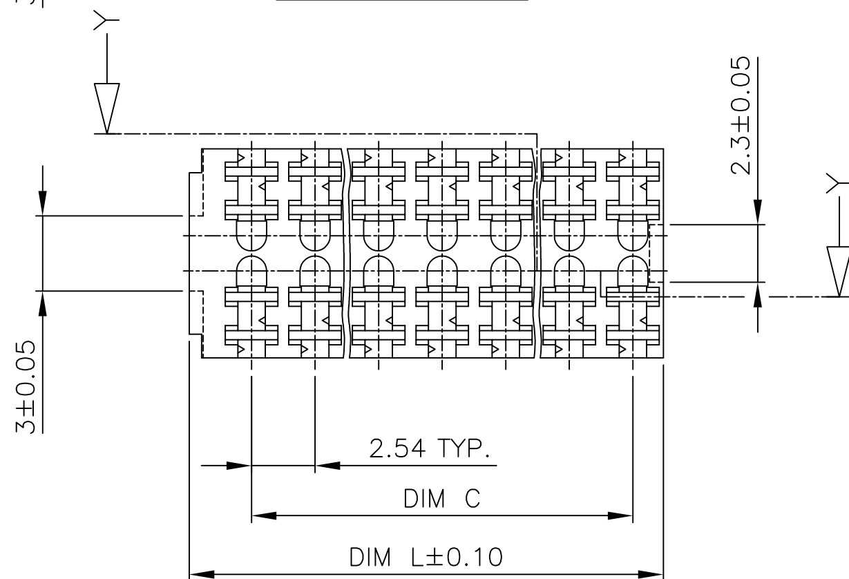
SECTION Y-Y
