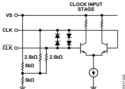
Figure 43. CLK Equivalent Input Circuit
