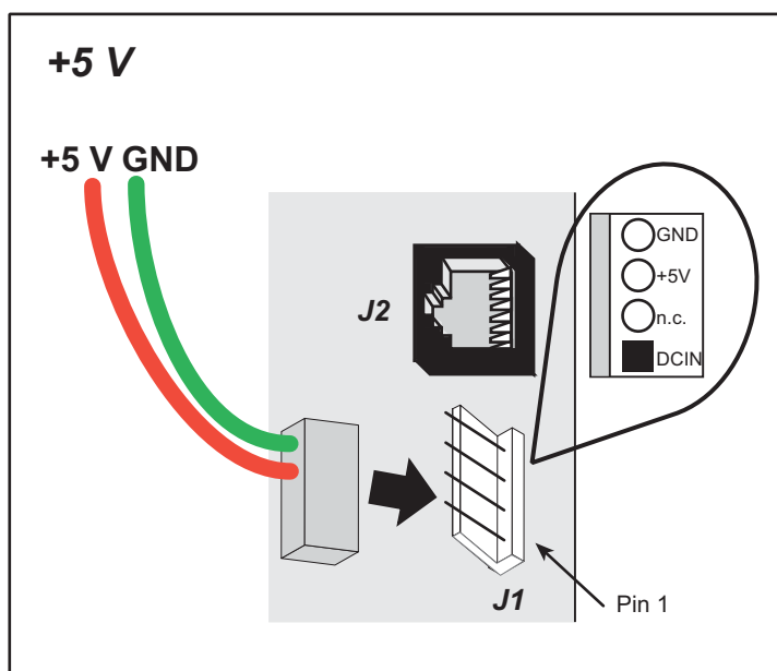
Figure 44. Power-Supply Connections
