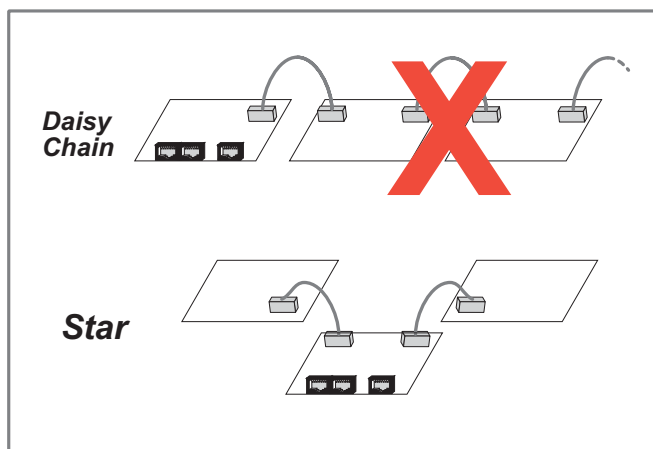
Figure 45. Daisy Chain vs. Star Configurations
