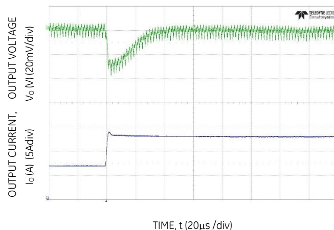
Figure 16. Transient Response to Dynamic Load Change from 50% to 100% at 12Vin, C_{out}=8 \times 47\mu\text{F} + 2 \times 330\mu\text{F} CTune=1.8nF, RTune=300Ω
