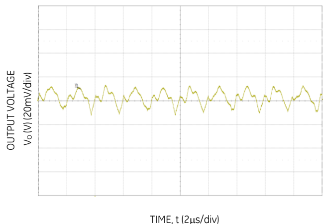
Figure 15. Typical output ripple and noise ( C_o=5 \times 22\mu\text{F} ceramic, V_{IN} = 12\text{V} , I_o = I_{o,max} ).
