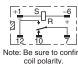
Terminal Arrangement/ Internal Connections (Bottom View)
