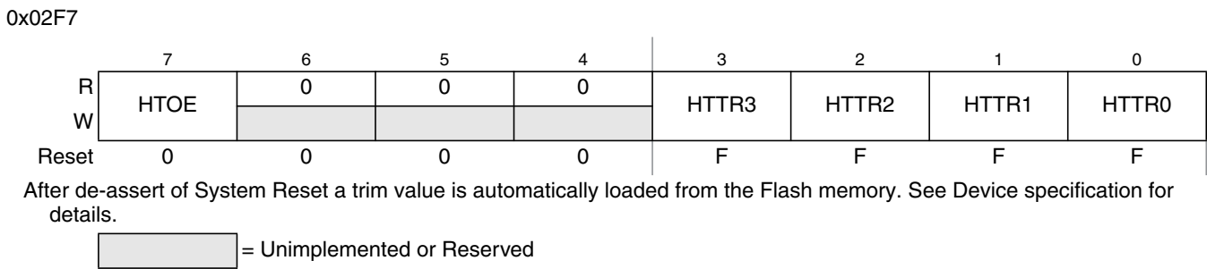
Figure 4-25. High Temperature Trimming Register (CPMUHTTR)
