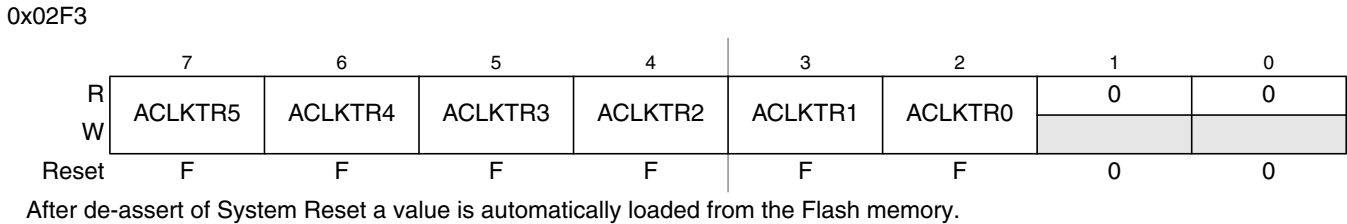
Figure 4-21. Autonomous Clock Trimming Register (CPMUACLKTR)
