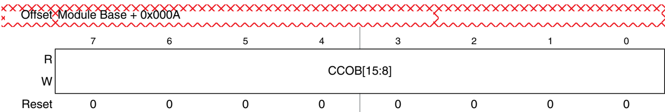
Figure 17-14. Flash Common Command Object High Register (FCCOBHI)
