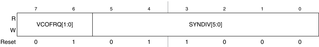
Figure 4-4. S12CPMU_UHV Synthesizer Register (CPMUSYNR)
