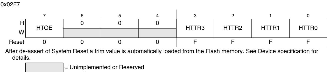
Figure 4-25. High Temperature Trimming Register (CPMUHTTR)
