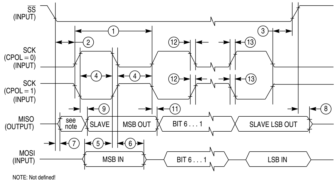
Figure K-5. SPI Slave Timing (CPHA=1)
