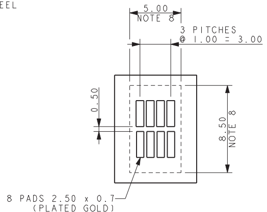
MATING PCB LAYOUT
