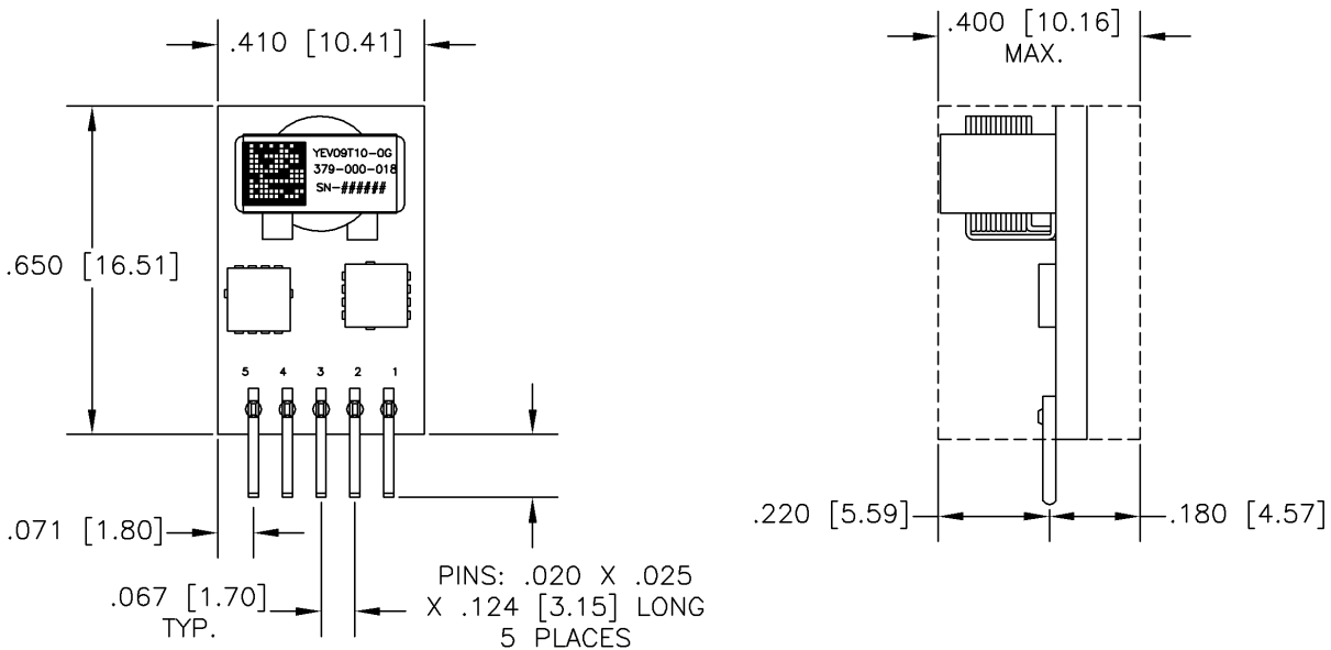
Figure 22. Mechanical Drawing
