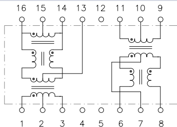
N2 Package
