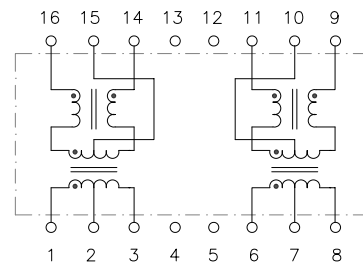
Circuit D
