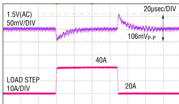
Figure 4. Load Step Response of the DC1632A at V_{IN} = 12V . C_{OUT} = 4 \times Sanyo 2R5TPE330M9 || 2 \times 100\mu\text{F X5R 6.3V 1206} , L1, 2 = 0.44 \mu H, f_{SW} = 300\text{kHz}
