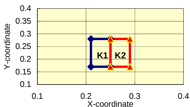
C. I. E. 1931 Chromaticity Diagram
