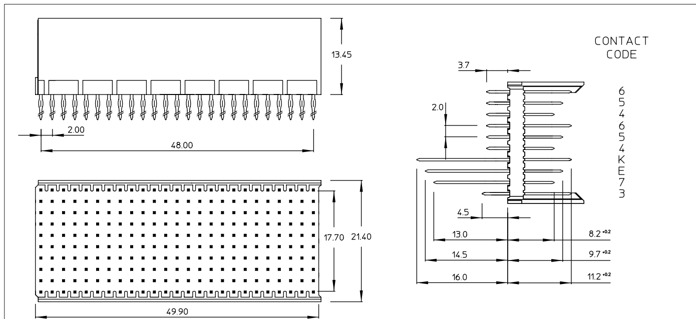
Standard loading patterns (seen from mating side)
