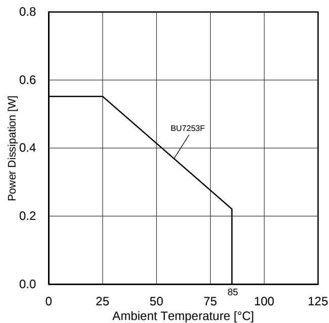
Figure 21. Power Dissipation vs Ambient Temperature (Derating Curve)
