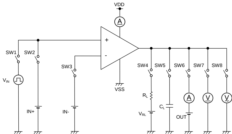
Figure 42. Test Circuit 2
