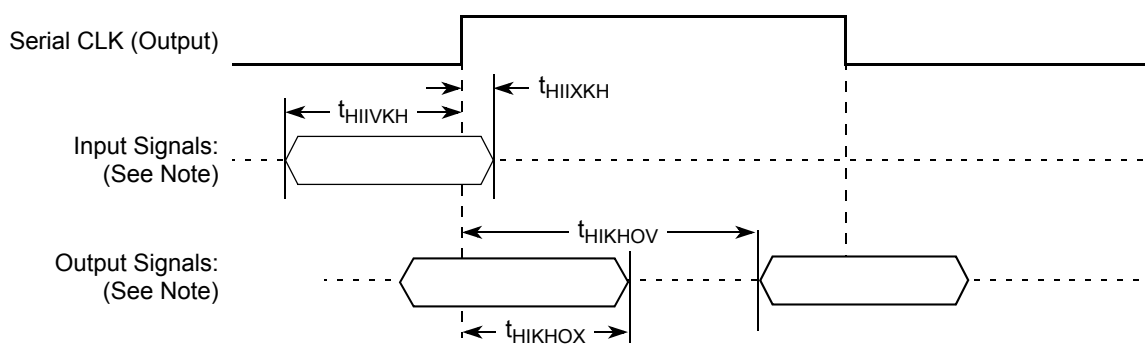
Figure 22. AC Timing (Internal Clock) Diagram
