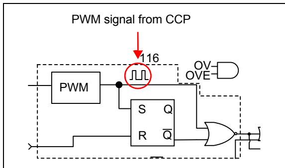
FIGURE 26-1: MCP19116/7 SNIPPET SHOWING SYSTEM CLOCK FROM PWM MODULE
