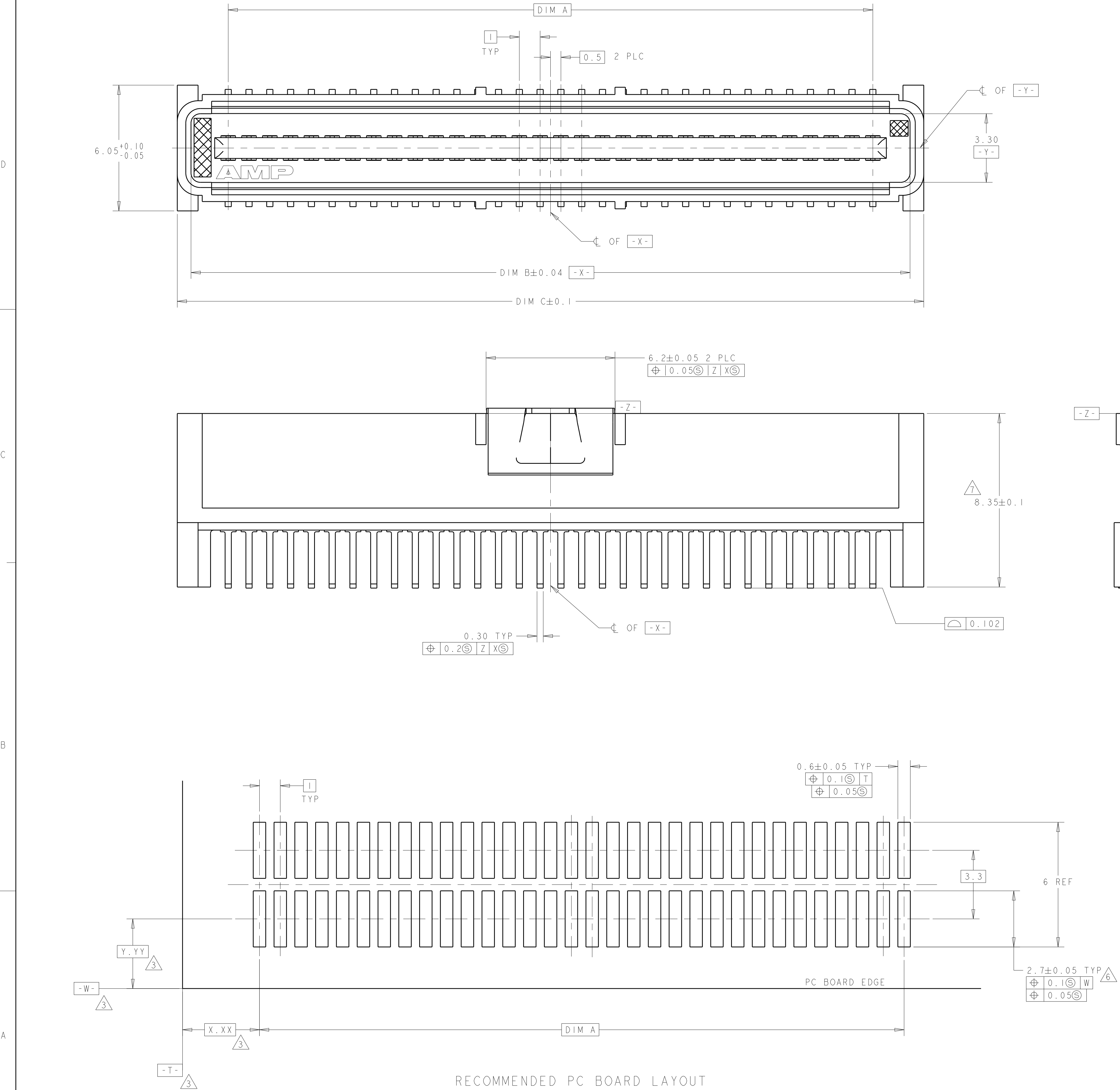
RECOMMENDED PC BOARD LAYOUT
