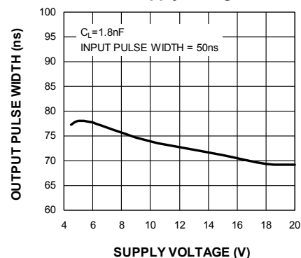
Pulse Stretching vs. Supply Voltage
