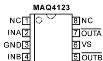
DUAL INVERTING
