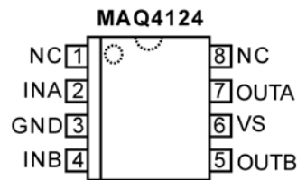
DUAL NON-INVERTING
