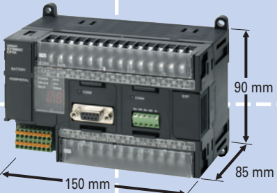
CP1H-□□ 40D□-□
