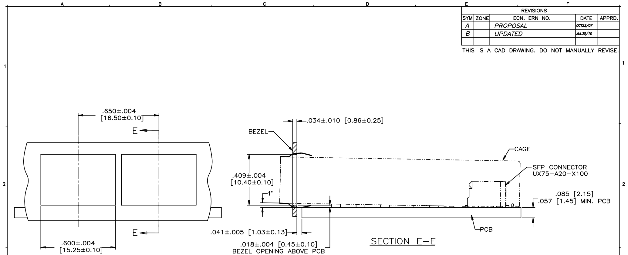
RECOMMENDED BEZEL DESIGN (ONE SIDE CAGE MOUNTING)
