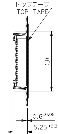
SECT. Z-Z
