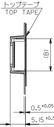
SECT. Y-Y
