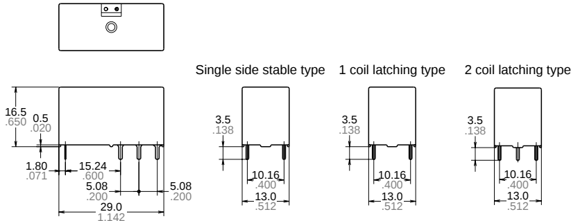
External dimensions
