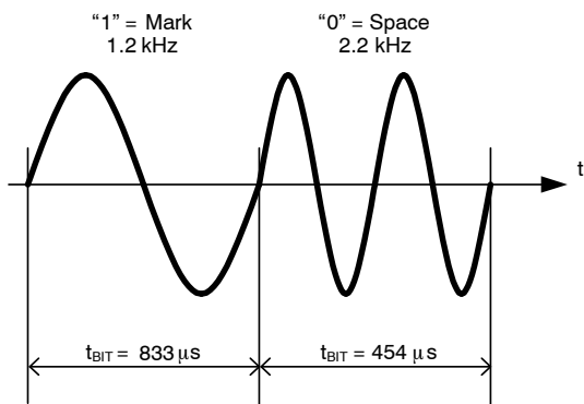
Figure 6. Modulation Timing
