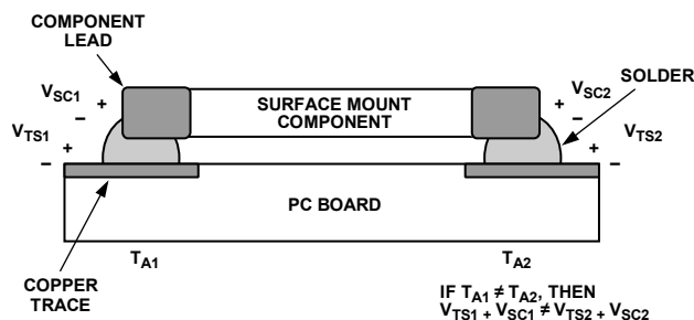
Figure 54. Mismatch in Seebeck Voltages Causes a Thermoelectric Voltage Error
