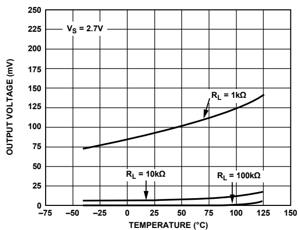
Figure 48. Output Voltage to Supply Rail vs. Temperature
