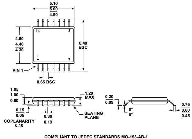
Figure 72. 14-Lead Thin Shrink Small Outline Package [TSSOP] (RU-14)
