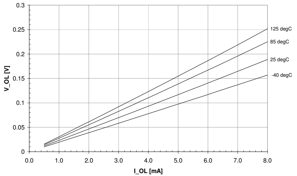
Figure 36-28. I/O Pin Output Voltage vs. Sink Current (25°C, DPDS0=1)
