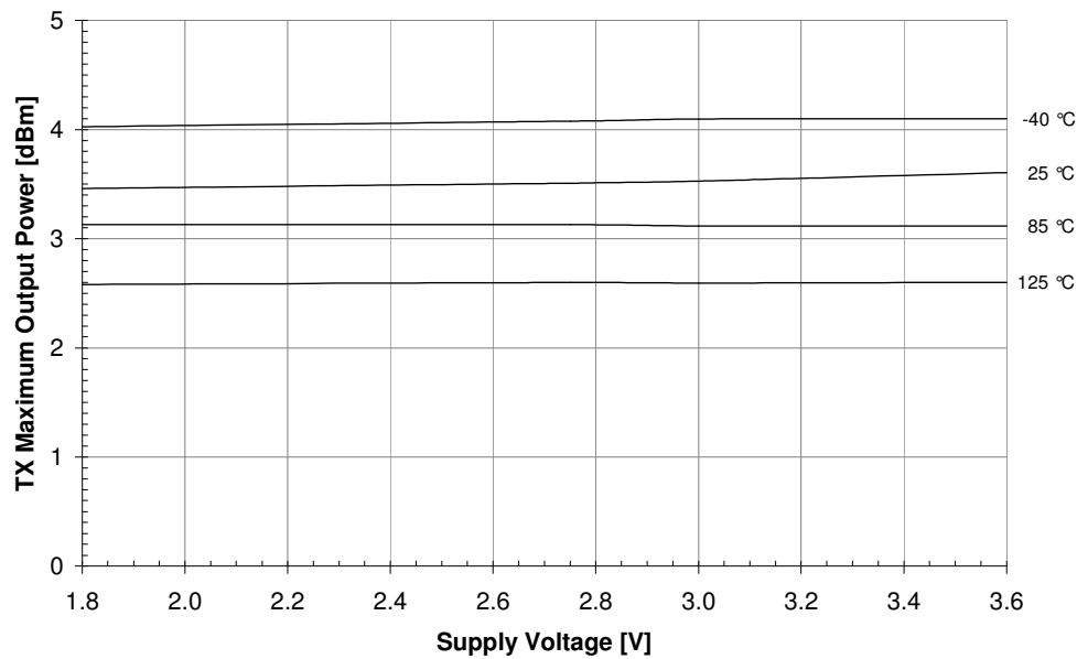
Figure 36-20. TX maximum output power
