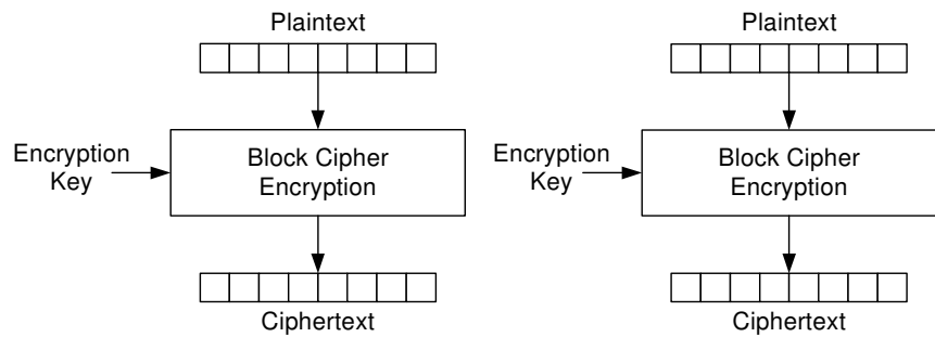
Figure 9-36. ECB Mode - Encryption
