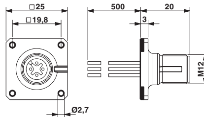
M12 flush-type plug
