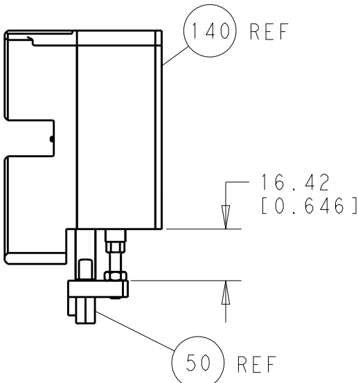
HOLDDOWN SET-UP
