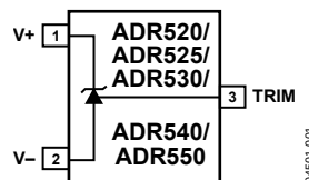
Figure 1. 3-Lead SC70 (KS) and 3-Lead SOT-23-3 (RT)
