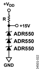
Figure 22. +15 V Output with Stacked ADR550s
